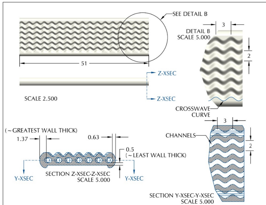
Figure 3 - CAD drawing with improved design of 8YSZ anode.
