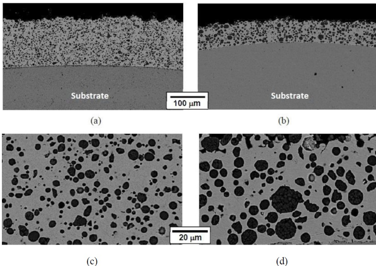
Figure 7 - SEM cross-sectional images of as-deposited NiCo-CrAlY coatings plated using powders with different particle sizes: (a) and (c) 5- \mu\text{m} particles; (b) and (d) 10- \mu\text{m} particles.
