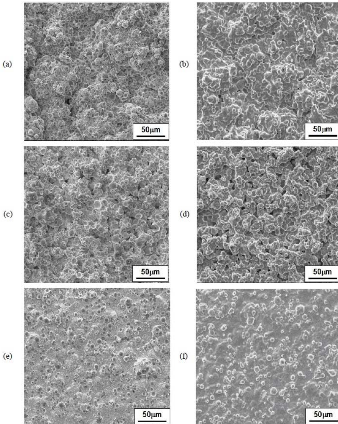
Figure 13 - SEM surface images of the specimens for oxidation tests before and after heat treatment:
