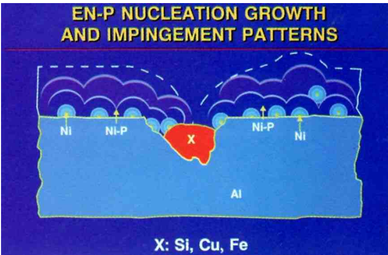
Figure 7 - Pore formation.
